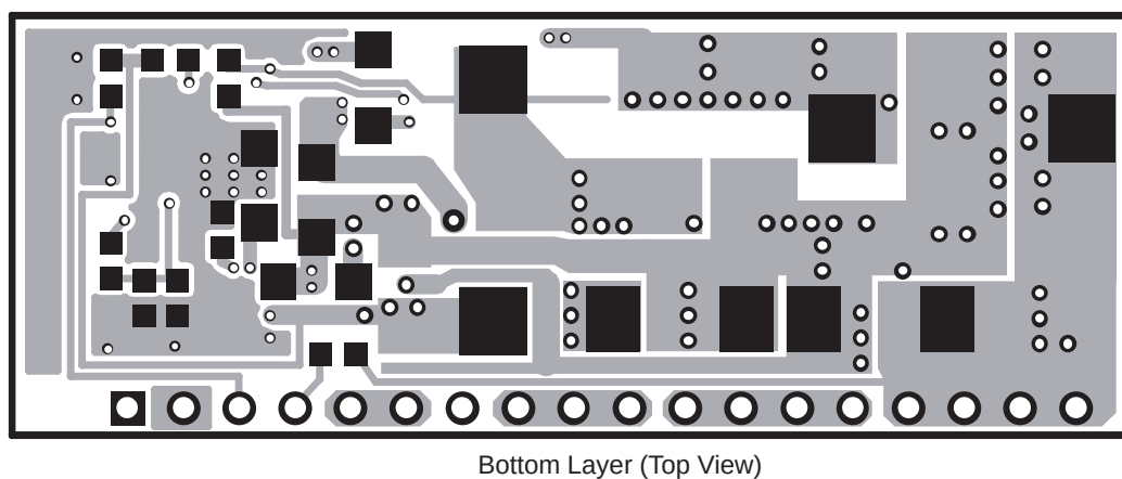
Figure 1–7. Bottom Layer (Top View)
