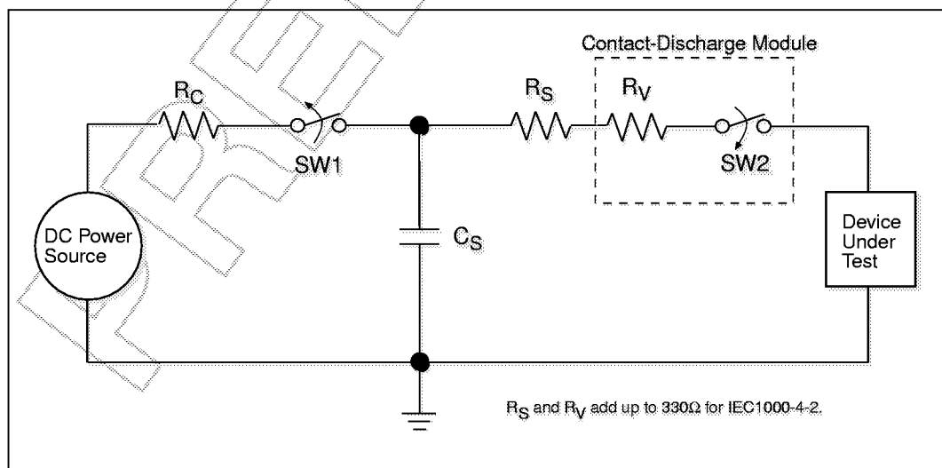
Figure 15. ESD Test Circuit for IEC1000-4-2
