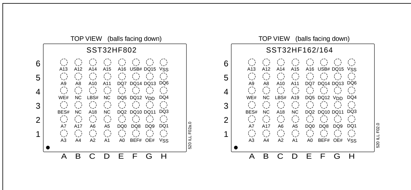
FIGURE 3: PIN ASSIGNMENTS FOR 48-BALL LFBGA (6MM X 8MM)
