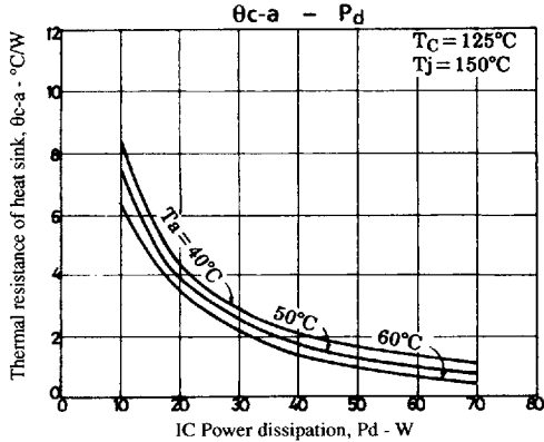
Figure 3. STK4162II θc-a - Pd
