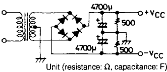
Specified Transformer Power Supply (Equivalent to RP-25)
