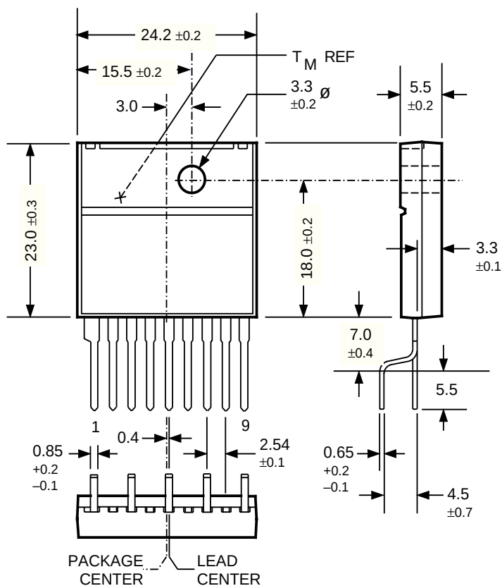
Dimensions in Millimeters (controlling dimensions)
