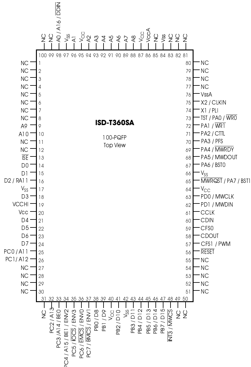
Figure 1-1: 100-PQFP Package Connection Diagram
