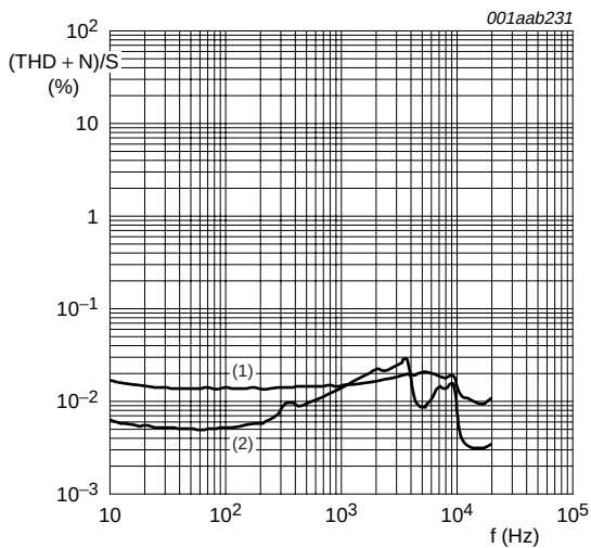
Fig 14. (THD + N)/S as a function of frequency; SE configuration with 2 × 3 Ω load.
