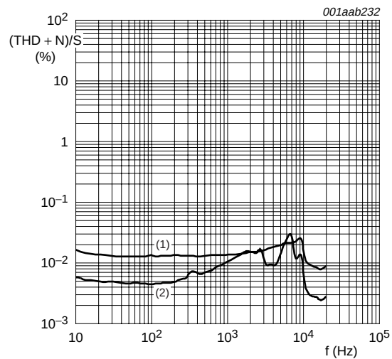
Fig 15. (THD + N)/S as a function of frequency; SE configuration with 2 × 4 Ω load.
