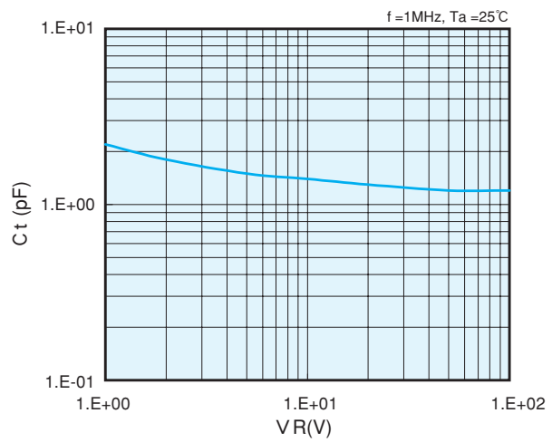
Diode Capacitance vs. Reverse Voltage
