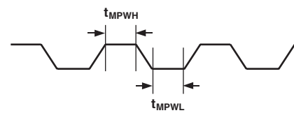
Figure 3. MCLK_IN Timing
