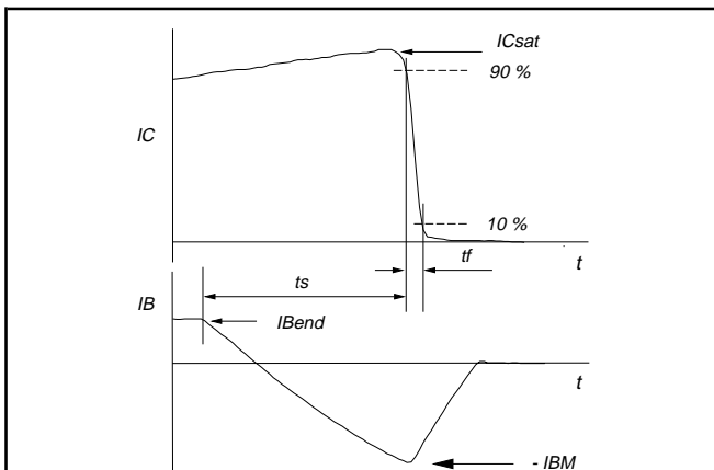
Fig.2. Switching times definitions.
