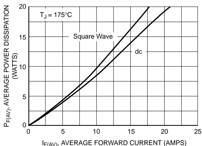
Figure 2. Power Dissipation
