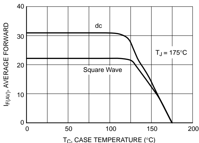
Figure 1. Current Derating
