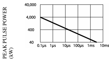
PULSE WIDTH
