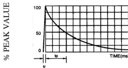
CURRENT PULSE WAVEFORM
