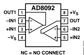
Figure 3. MSOP-8 and SOIC-8 (RM-8, R-8)
