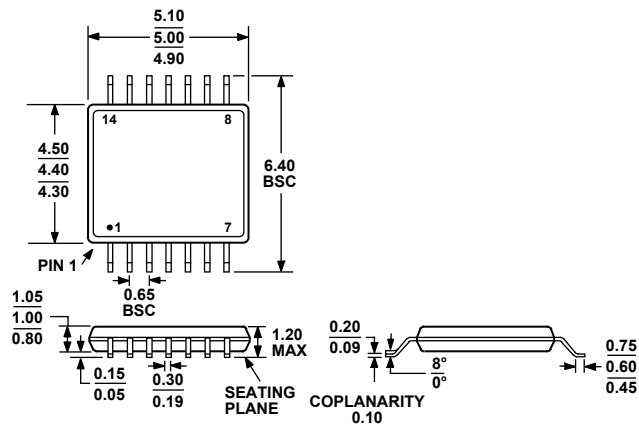
Figure 38. 14-Lead Standard Small Outline Package [TSSOP] (RU-14) Dimensions shown in millimeters
