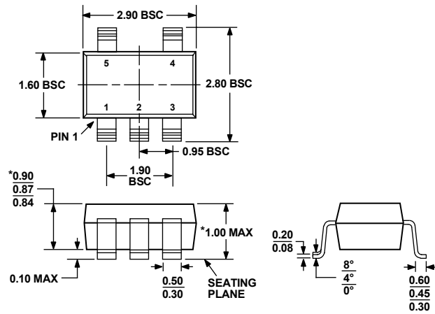
Figure 36. 5-Lead Thin Small Outline Transistor Package [TSOT] (UJ-5)
