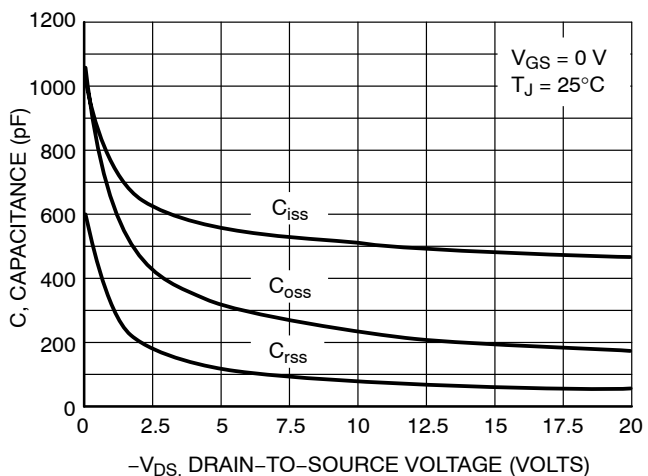
Figure 6. Capacitance Variation
