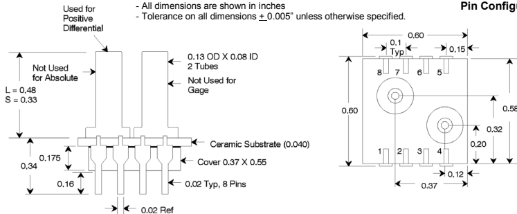
Pin Configuration
