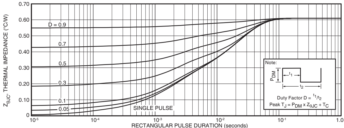
FIGURE 24a. MAXIMUM EFFECTIVE RECTANGULAR PULSE DURATION, JUNCTION-TO-CASE vs. PULSE DURATION RC MODEL
