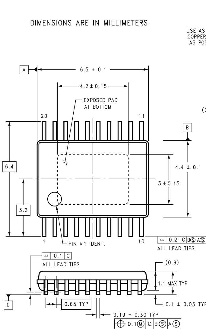
20-Lead Molded TSSOP, Exposed Pad, 6.5x4.4x0.9mm Order Number KB4863MTE Package Number MXA20A
