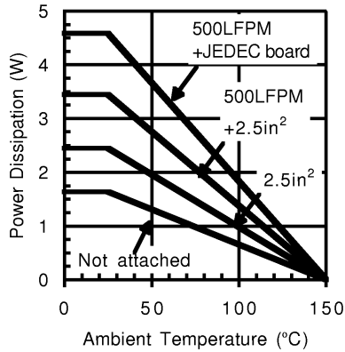
KB4863MTE (Note 17) Power Derating Curve
