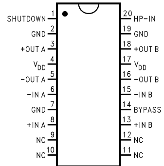
Top View Order Number KB4863MT MTC20 for TSSOP
