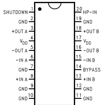
Top View Order Number KB4863MTE MXA20A for Exposed-DAP TSSOP
