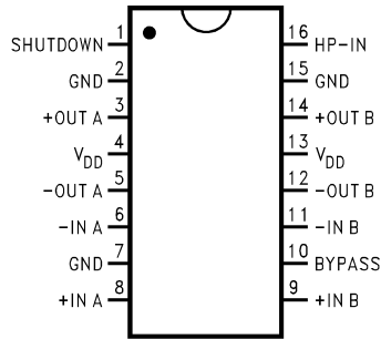
Top View Order Number KB4863M, KB4863N M16B for SO N16E for DIP
