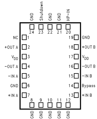
Top View Order Number KB4863LQ LQA24A for Exposed-DAP LLP
