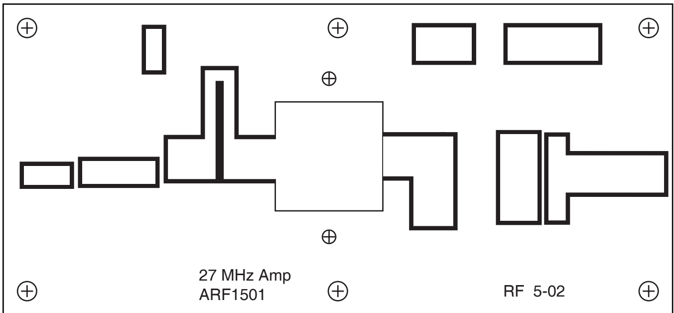
1:1 pcb artwork
