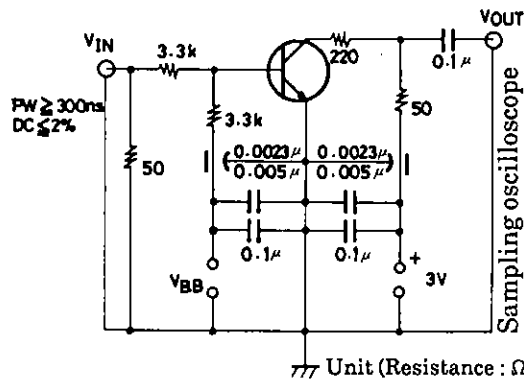
t_{on}, t_{off} Test Circuit
