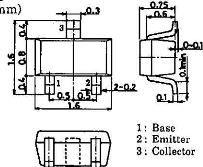
Package Dimensions 2106A (unit: mm)
