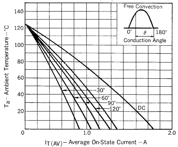
Fig. 6 T_a-I_{T(AV)} RATING
