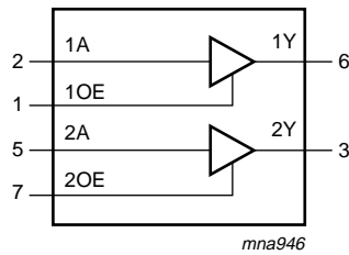
Fig 1. Logic symbol.
