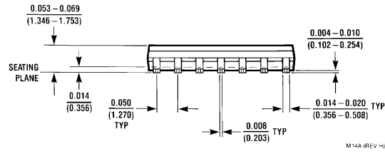
14-Lead (0.150" Wide) Small Outline Integrated Circuit Package Number M14A
