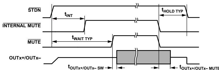
Figure 3. Timing Diagram (Typical)
