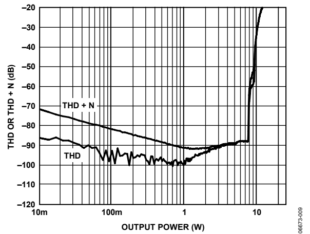
Figure 9. THD or THD + N vs. Output Power, 6 Ω, PVDD = 12 V
