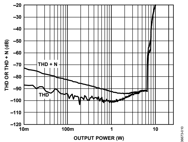
Figure 10. THD or THD + N vs. Output Power, 8 Ω, PVDD = 12 V
