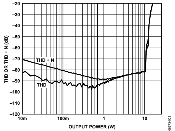
Figure 8. THD or THD + N vs. Output Power, 4 Ω, PVDD = 12 V
