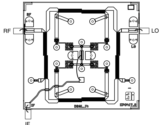
Requires two IF bonds. LO to IF isolation is degraded by 7 dB for this configuration.
