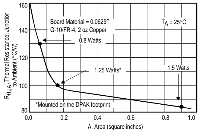
Figure 8. Thermal Resistance versus Collector Pad Area for the SOT-223 Package (Typical)
