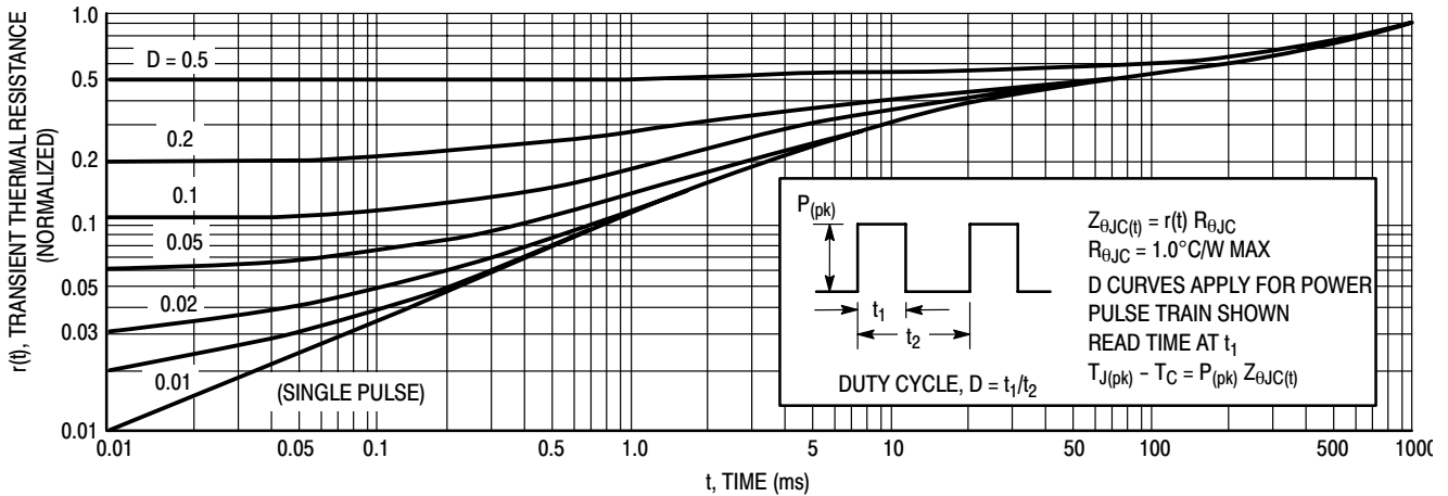
Figure 7. Thermal Response
