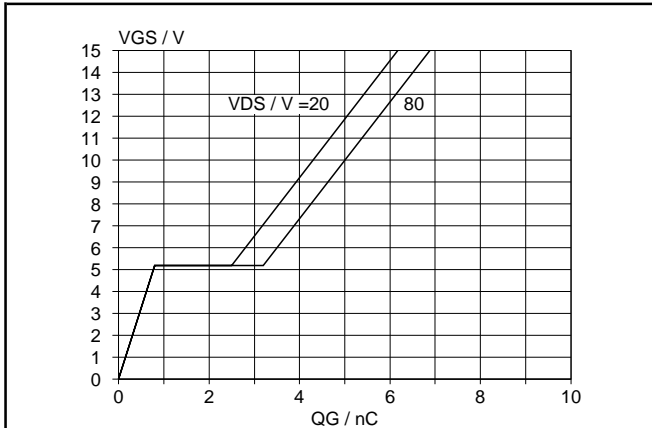
Fig.13. Typical turn-on gate-charge characteristics. V_{GS} = f(Q_G) ; conditions: I_D = 1\text{ A} ; parameter V_{DS}
