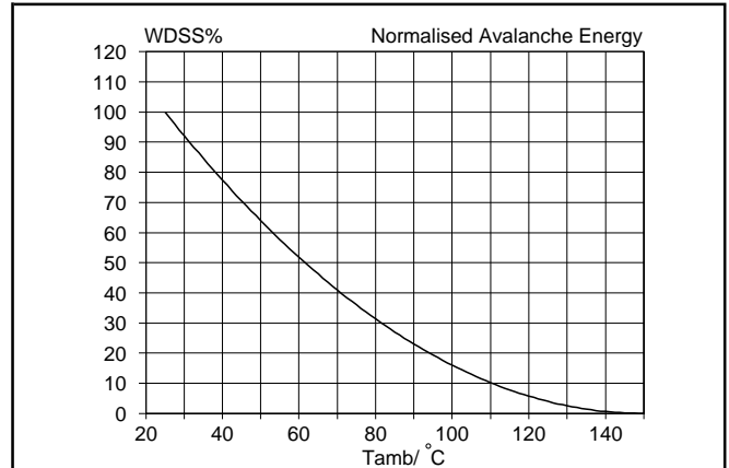
Fig.15. Normalised avalanche energy rating. W_{DSS}\% = f(T_{amb}) ; conditions: I_D = 1\text{ A}
