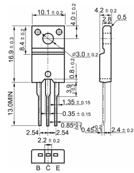
TO-220F
