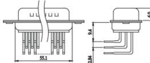
50 POSITION MALE
