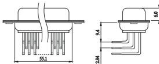
50 POSITION FEMALE
