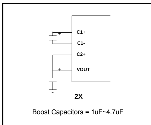
Figure 16 Capacitor Connections
