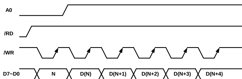
Write Timing Diagram
