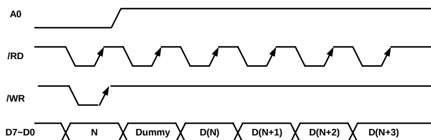
Read Timing Diagram
