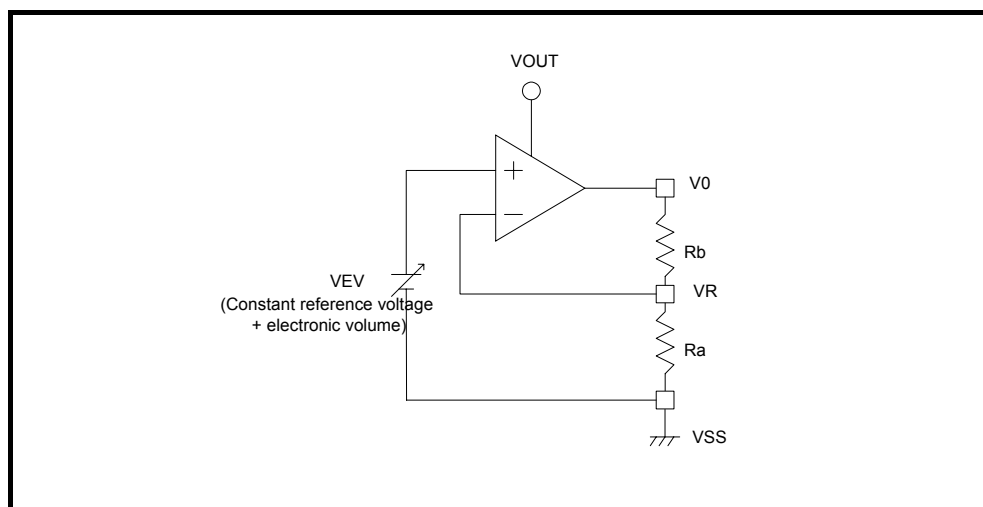
Figure 17 Resistor Connections
