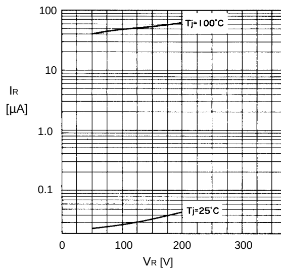
Reverse characteristics
