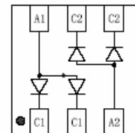
FBAT54ADW Marking:KL6
