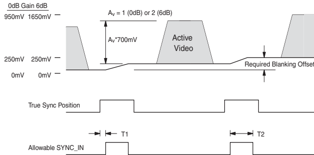
Figure 13. Bi-Level External Sync Clamping and Bias
