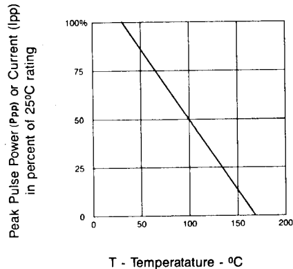
FIGURE 3 DERATING CURVE
