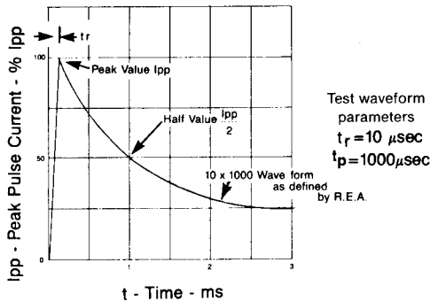
FIGURE 2 PULSE WAVE FORM
