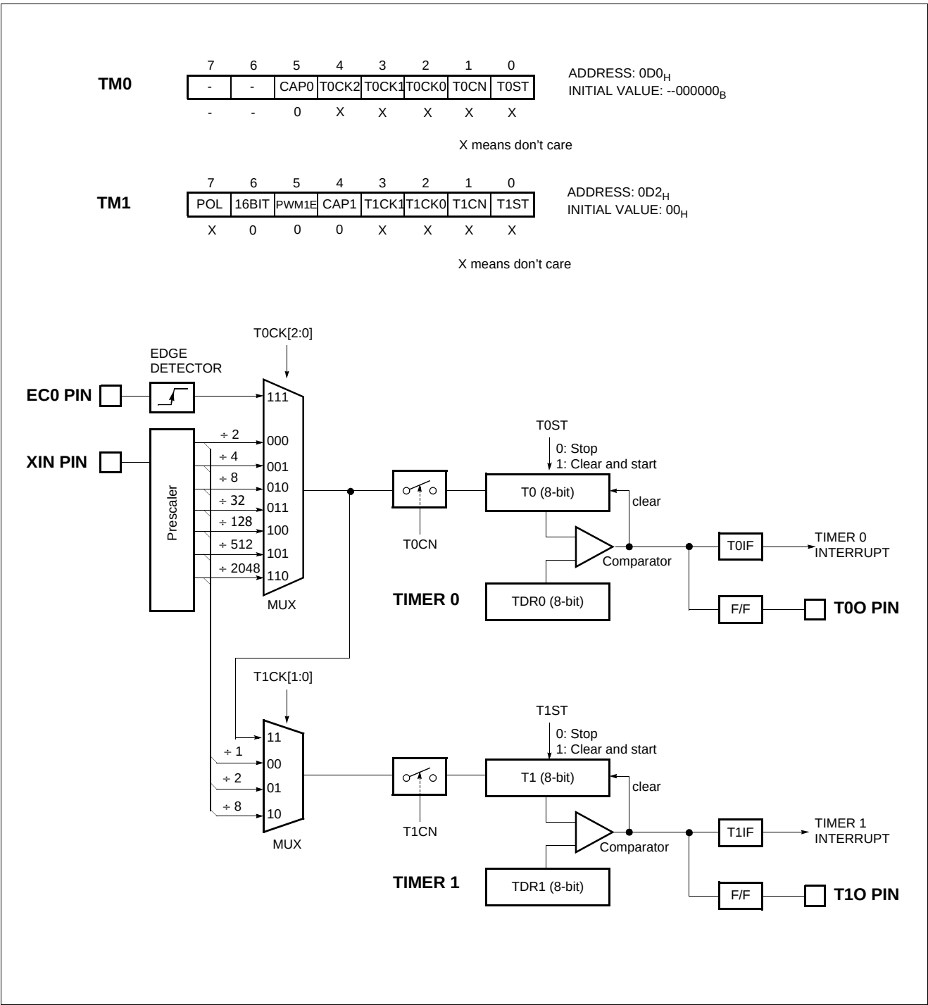
Figure 12-2 8-bit Timer/Counter 0, 1
