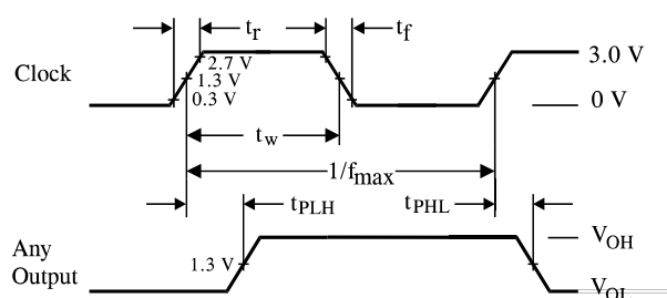
Figure 1. Switching Waveform
