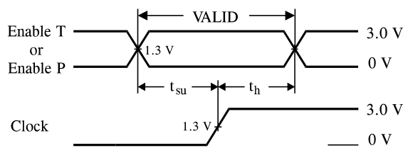
Figure 4. Switching Waveform
