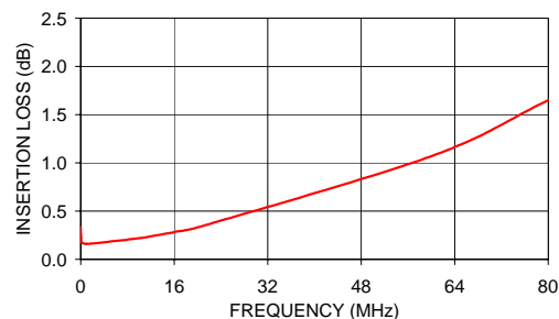
JT-1975 INSERTION LOSS
