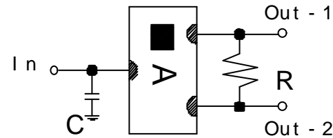
850/950 MHz Chip Multilayer Splitter/Combiner "FSLH-S090C"
