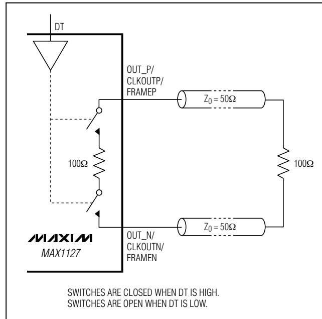
Figure 8. Double Termination
