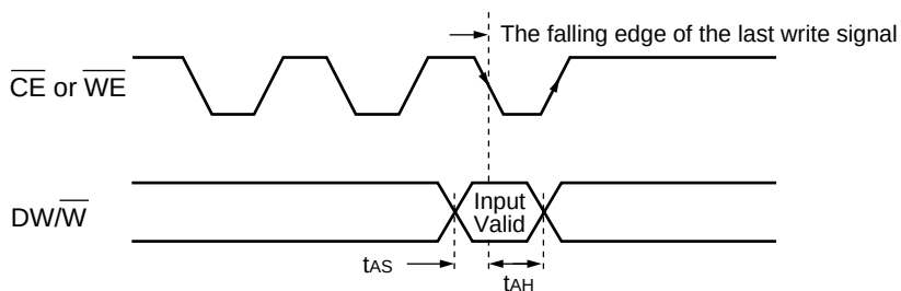
Figure 14 DW/\overline{W} Timing Diagram for Write Operations
