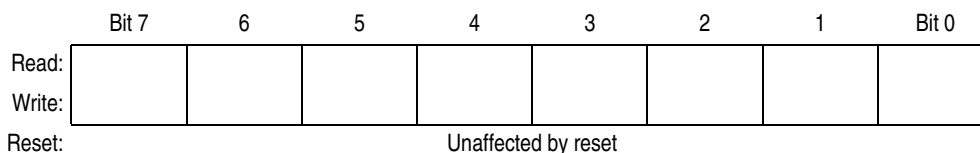
Figure 6-2. Accumulator (A)
