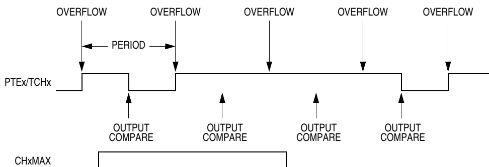
Figure 11-8. CHxMAX Latency
