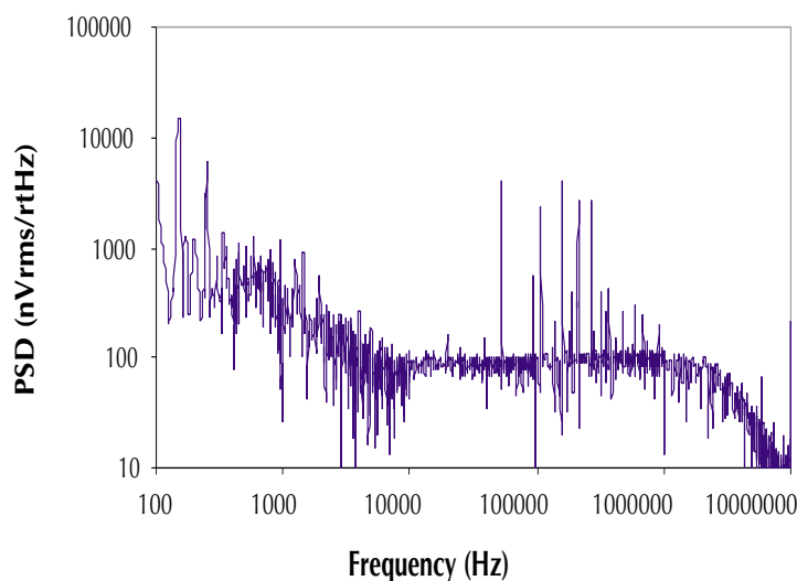
Figure 3. Transmit Regulator Noise Floor
