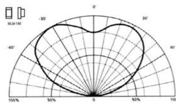
Directive Characteristics
