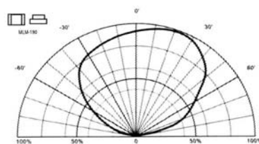
Directive Characteristics
