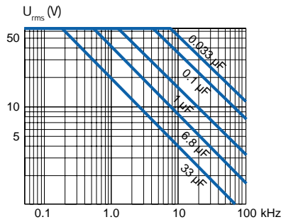
MMK7.5 ... 37.5 100/63
