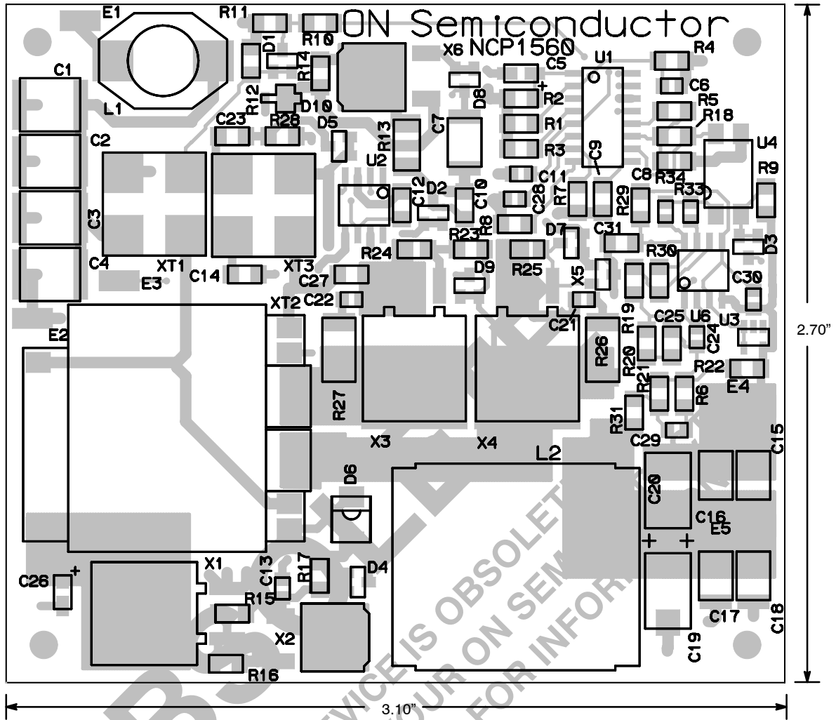
Figure 36. Board Arrangement
