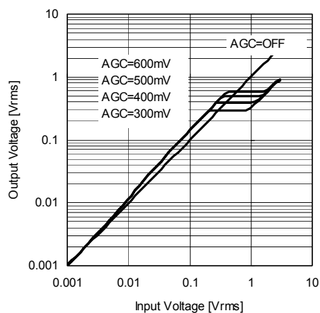
AGC Output Voltage vs. Input Voltage Ta=25°C, V+=9V, R L =47kΩ, Vin(A+Bch), f=1kHz, Vout(Ach), BW=400Hz-30kHz, VOL=0dB, BAL=0dB, BASS=TREB=0dB, BBE=OFF, Surround=OFF
