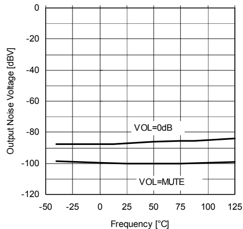
Output Noise Voltage (OUT) vs. Frequency V+=9V, R L =47kΩ, BAL=0dB, AGC=OFF, BASS=TREB=0dB, BBE=OFF, Surround=OFF
