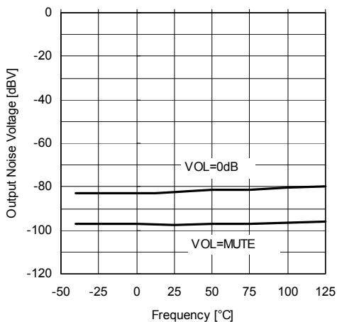
Output Noise Voltage (LINE) vs. Frequency V+=9V, R L =47kΩ, BAL=0dB, AGC=OFF, BASS=TREB=0dB, BBE=OFF, Surround=OFF
