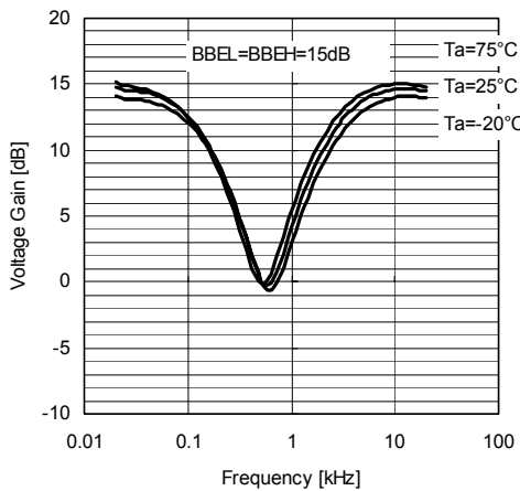
Voltage Gain vs. Frequency (BBE)
