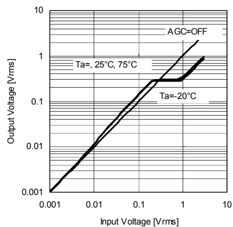
AGC Output Voltage vs. Input Voltage V+=9V, R L =47kΩ, Vin(A+Bch), f=1kHz, Vout(Ach), BW=400Hz-30kHz, VOL=0dB, BAL=0dB, AGC=300mV, BASS=TREB=0dB, BBE=OFF, Surround=OFF
