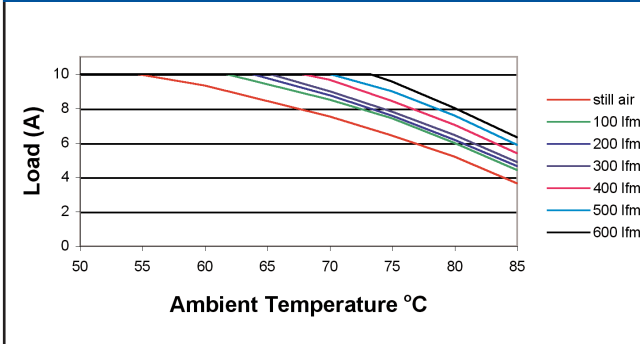
V_{OUT} = 1.2V
