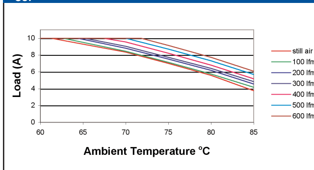
V_{OUT} = 2.0V
