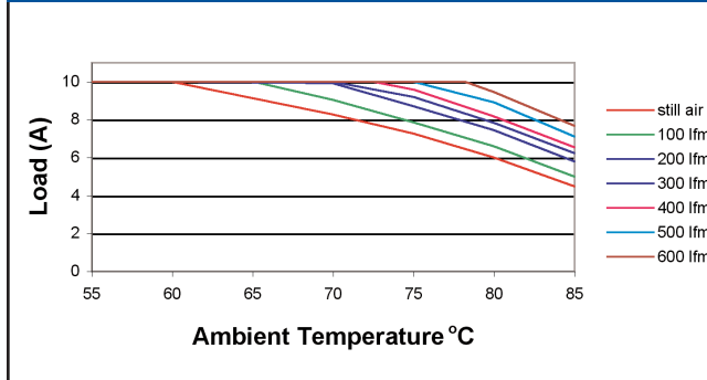
V_{OUT} = 1.5V
