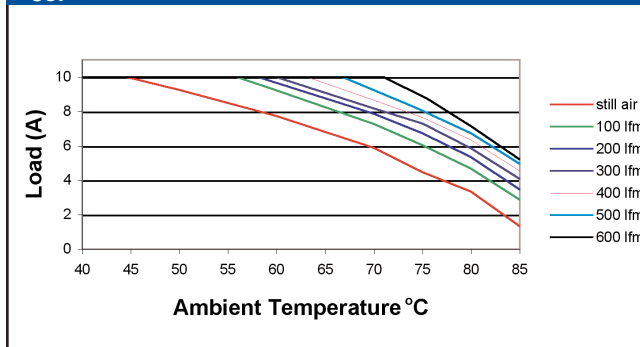
V_{OUT} = 3.3V
