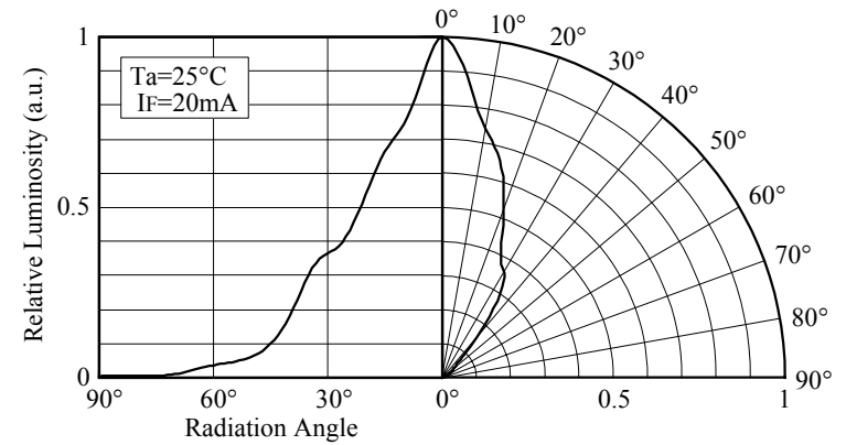
■ Directivity (NSPB520S)
