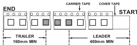
Tape Leader and Trailer Dimensions
